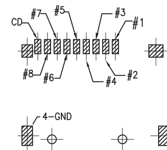
PIN ASSIGNMENT
