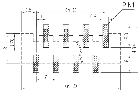
RECOMMENDED PCB LAYOUT (TOP VIEW) Tolerance: ±0.05
