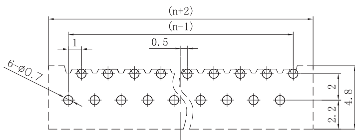
RECOMMENDED PCB LAYOUT (TOP VIEW) Tolerance: \pm 0.05
