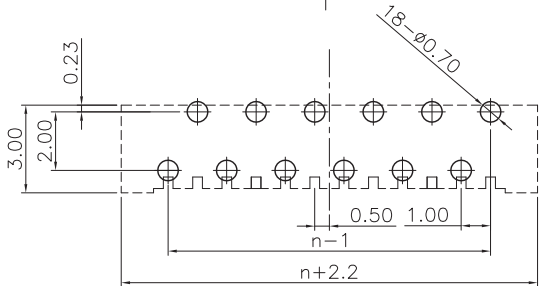
RECOMMENDED PCB LAYOUT (TOP VIEW) Tolerance: ±0.05
