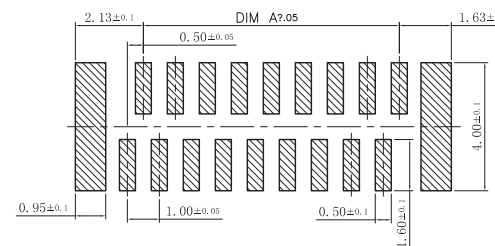
RECOMMENDED PCB LAYOUT(EVEN PIN) GENERAL TOLERANCE:±0.05(TOP VIEW)
