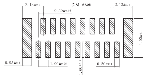
RECOMMENDED PCB LAYOUT(ODD PIN) GENERAL TOLERANCE:±0.05(TOP VIEW)
