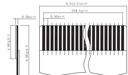
COMPLIANT FFC/FPC
