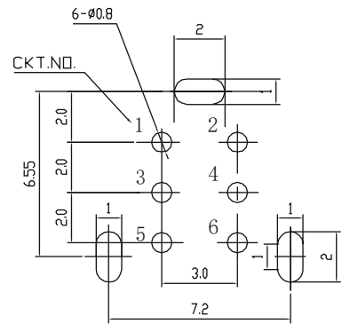
PCB BOARD LAYOUT
