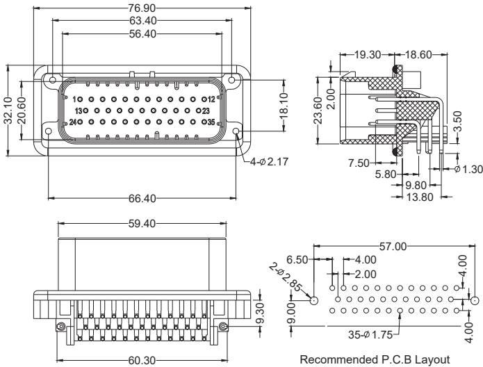
R/A ANGLE
