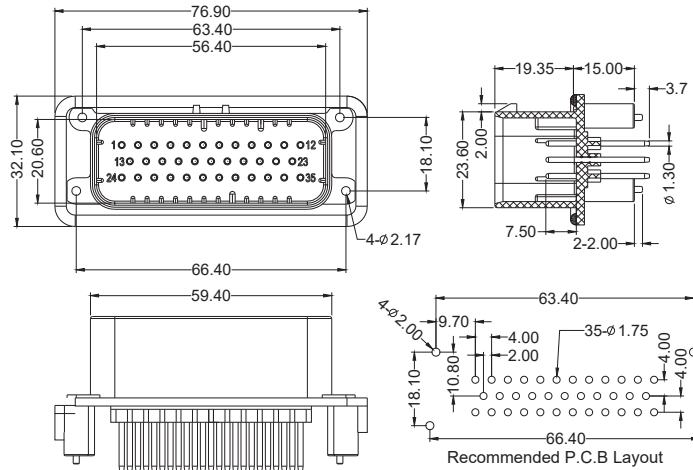
STRAIGHT
