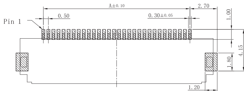
RECOMMEND PCB LAYOUT
