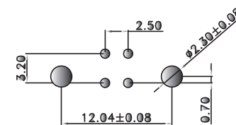
RECOMMENDED P.C.B. PATTERN LAYOUT
