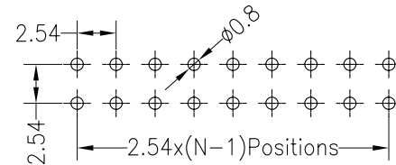
Recommended P.C.B Layout(Top Side) (PCB BOARD TOLERANCE±0.05)
