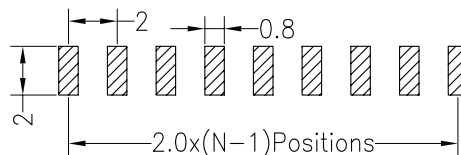
Recommended P.C.B Layout(Top Side) (PCB BOARD TOLERANCE±0.05)
