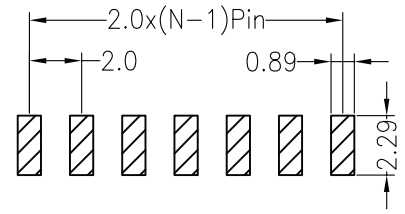
Recommended P.C.B Layout(Top Side) (PCB BOARD TOLERANCE±0.05)
