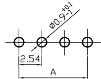
P. C. B LAYOUT
