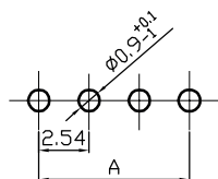
P. C. B LAYOUT
